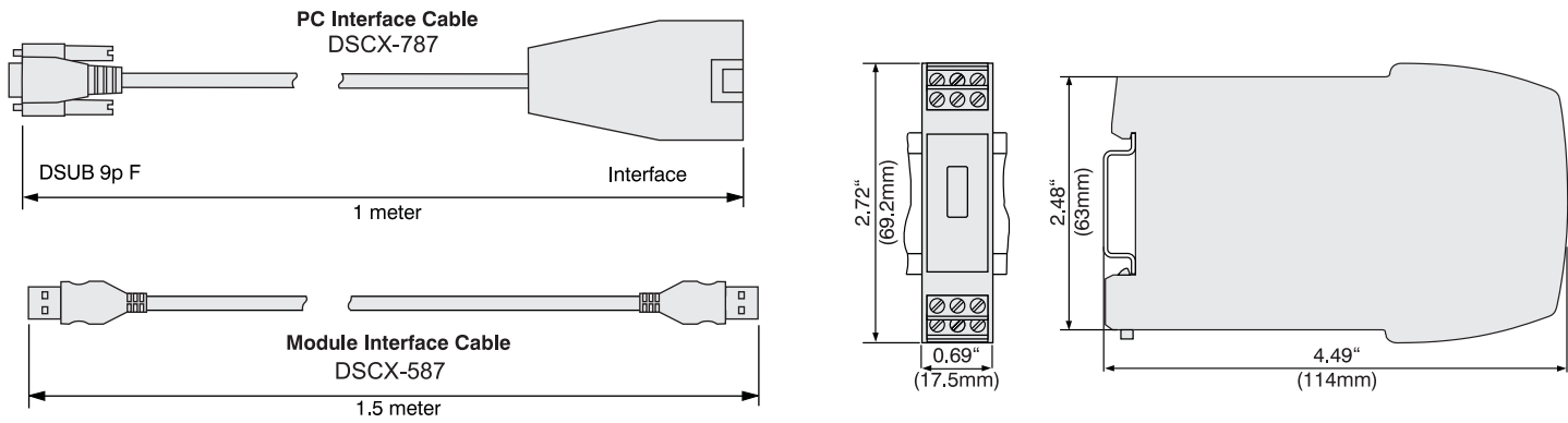
Figure 4: Product Dimensions
