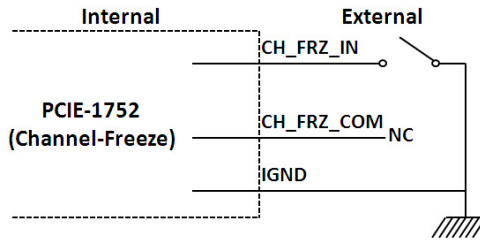
Figure 3.5: Wiring in dry contact input mode
