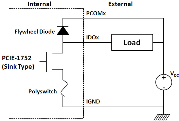
Figure 3.3: Isolated Digital Output Connection
