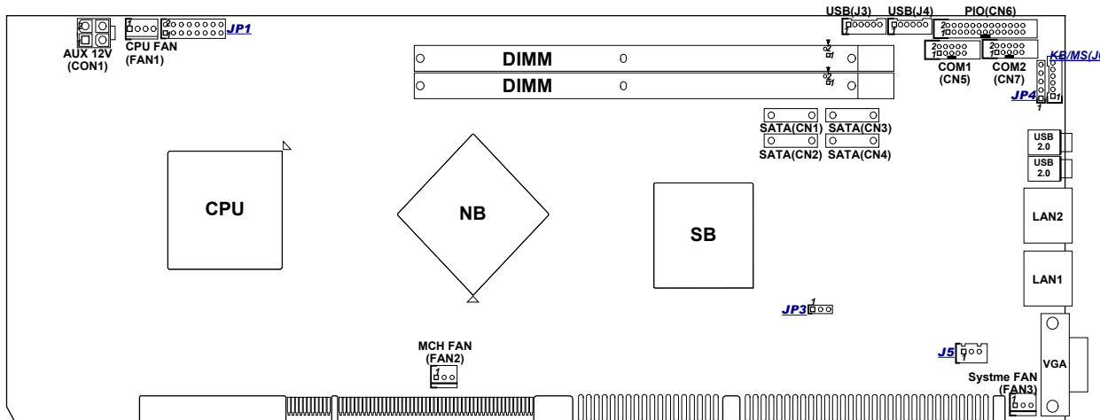
Figure 2-1: Jumper Location of PEAK 765VL2
