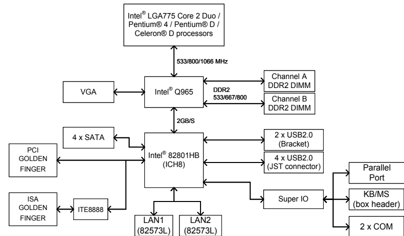
Figure 1.1 : Block Diagram of PEAK765VL2
