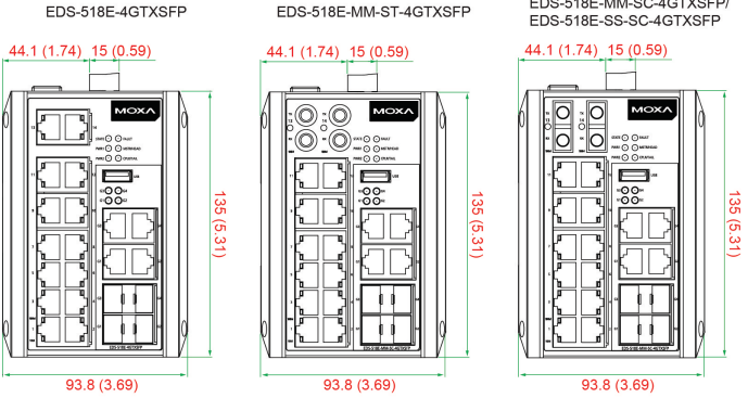
Front Views
