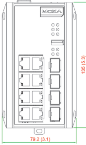
Front Views
